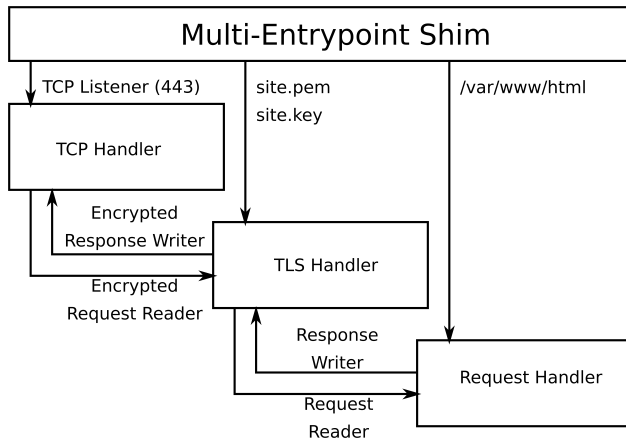
Figure 4. Process separation in a TLS server.
