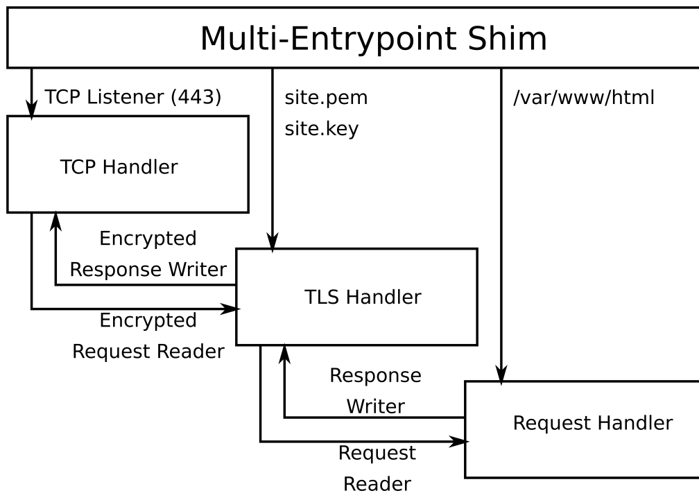
Figure 5.1: Process separation in a TLS server.
