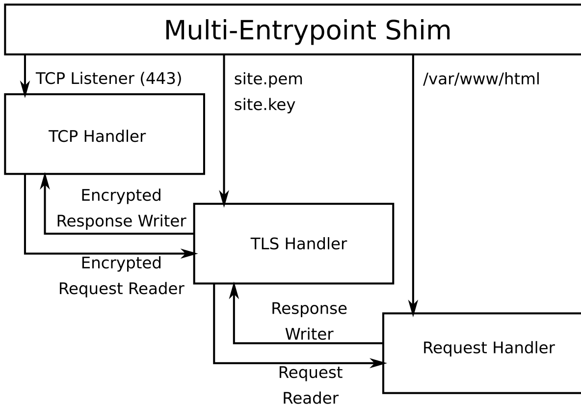
Figure 5.1: Process separation in a TLS server.
