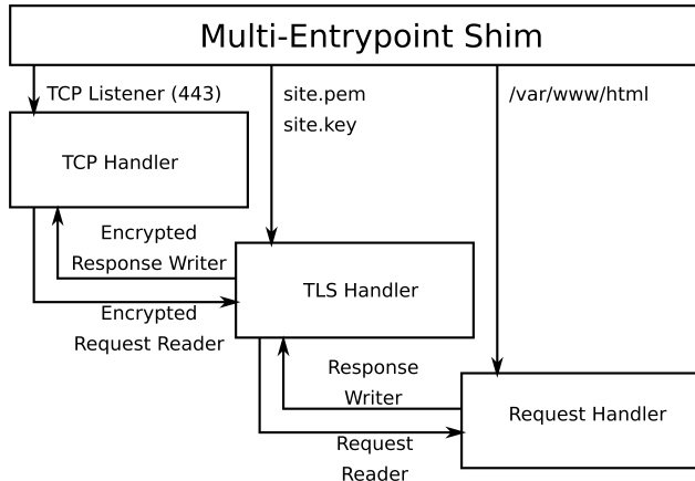
Figure 7. Process separation in a TLS server.
