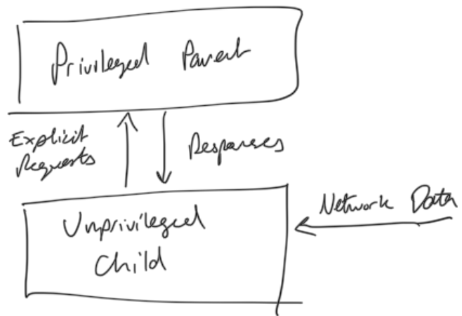
Figure 2. Data flow with the two processes in OpenBSD's privilege separated syslogd design.
