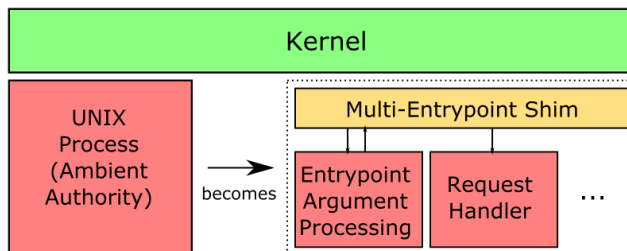
Figure 6. Interaction between the application and the environment.
